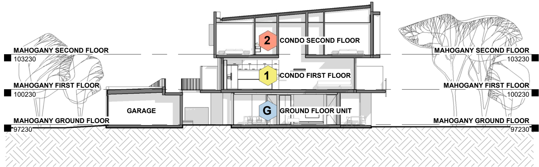
MAHOGANY BLOCK - TYPICAL SECTION SCALE 1 : 200
