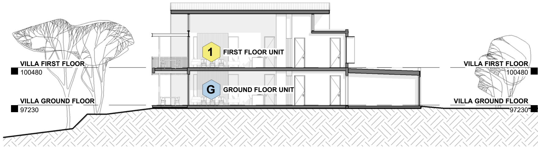
2 BEDROOM VILLA - TYPICAL SECTION SCALE 1 : 200
